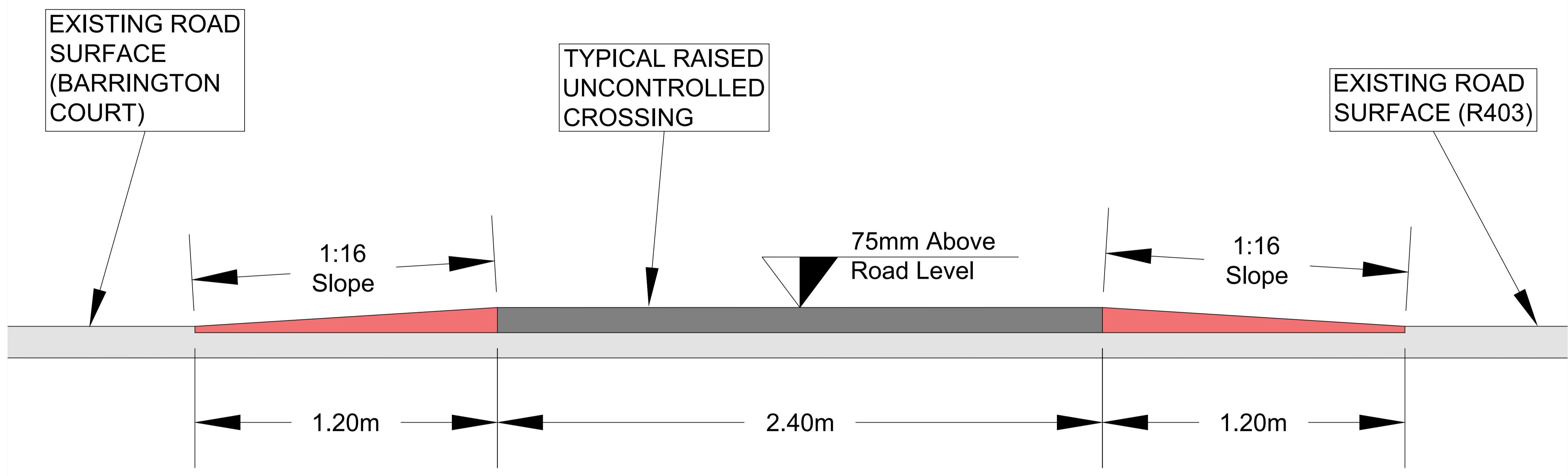
01 Section A-A 1002 Not To Scale
