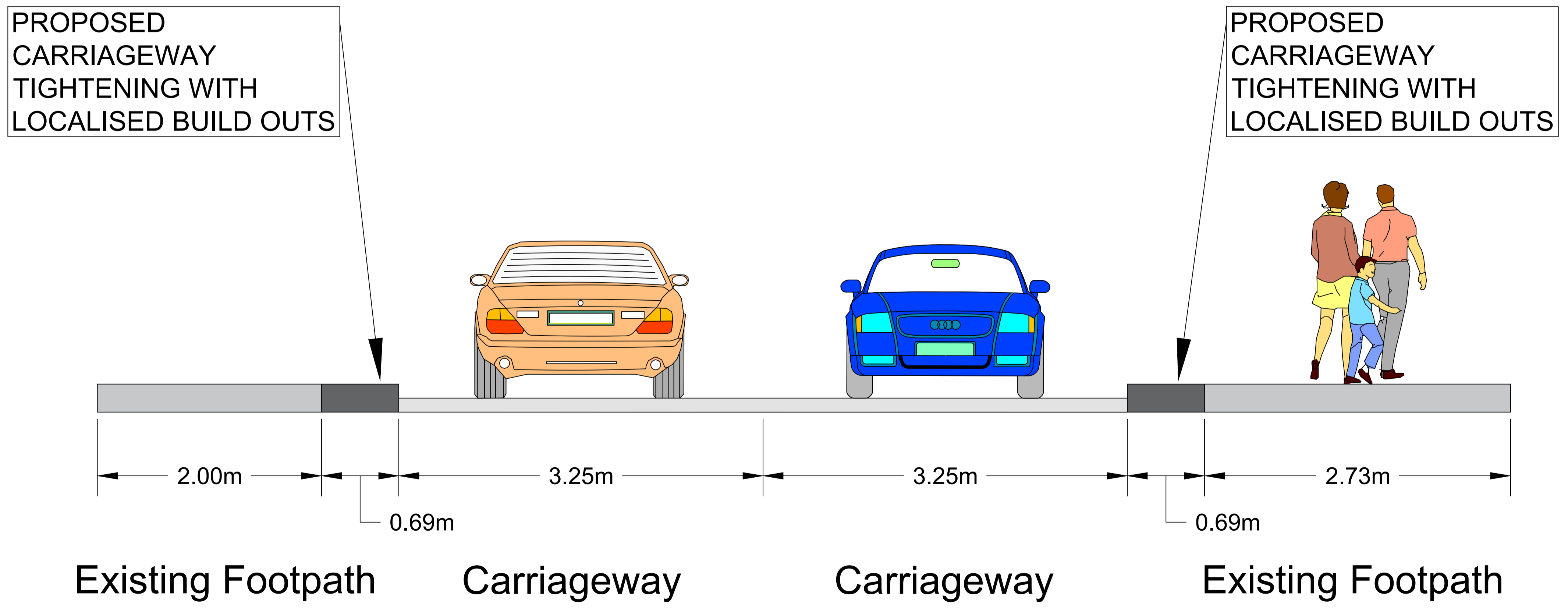
02 Section B-B 1005 Not To Scale
